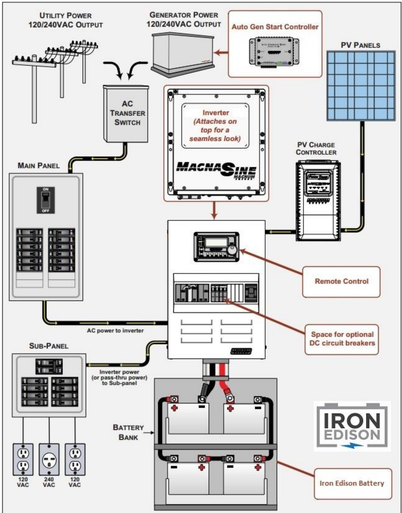
Simplified Installation Diagram
